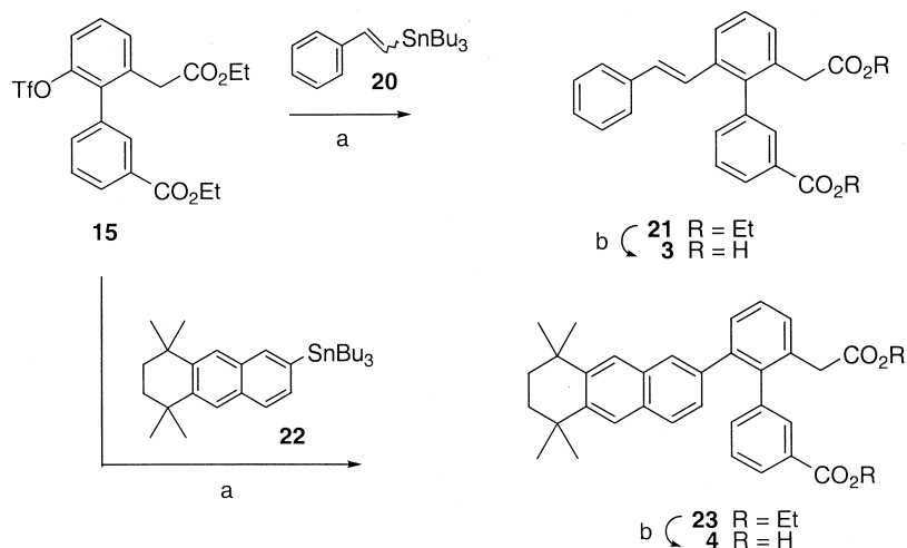
Scheme 4. Reaction conditions: (a) \text{PdCl}_2(\text{PPh}_3)_2 , LiCl, DMF, 110 °C; (b) 2 N NaOH, CH 3 OH, THF, reflux, then 1 N HCl.
