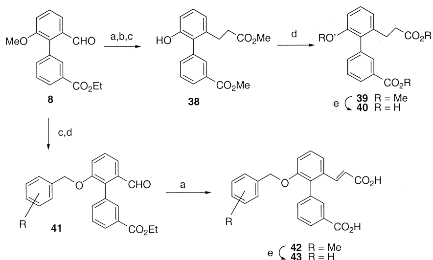
Scheme 7. Reaction conditions: (a) (\text{EtO})_2\text{P}(\text{O})\text{CH}_2\text{CO}_2\text{Me} (1.33 equiv), \text{NaOCH}_3 (2.5 equiv) in \text{CH}_3\text{OH} , toluene; (b) 10% \text{Pd/C} , \text{H}_2 (50 psi), \text{EtOH} ; (c) \text{Me}_2\text{BBr} , \text{ClCH}_2\text{CH}_2\text{Cl} ; (d) \text{ArCH}_2\text{OH} , DIAD, \text{PPh}_3 , THF, 0^\circ\text{C} ; (e) 2 N \text{NaOH} , \text{CH}_3\text{OH} , THF, reflux, then 1 N \text{HCl} .
