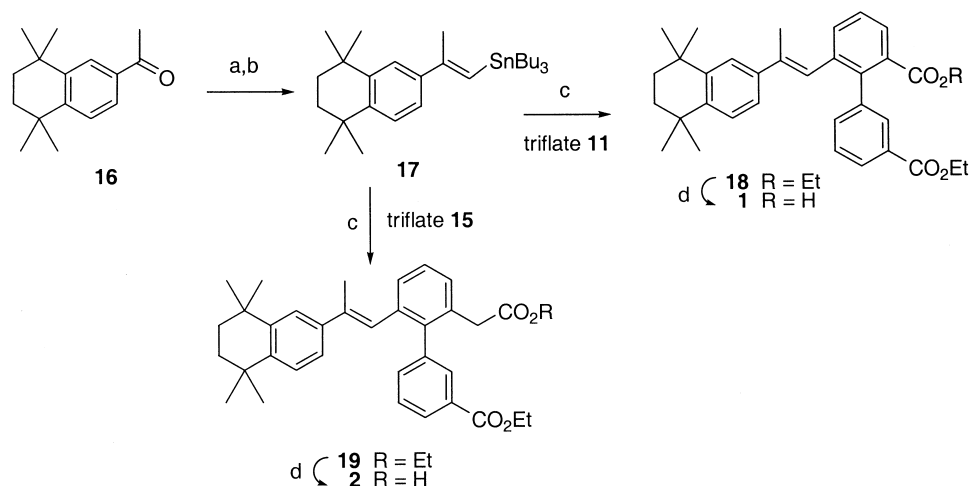
Scheme 3. Reaction conditions: (a) \text{Ph}_3\text{PCH}_2\text{Br} + \text{Br}^- , t -BuOK, THF, 0 °C; (b) t -BuLi, THF, –78 °C, then n -Bu 3 SnCl; (c) \text{PdCl}_2(\text{PPh}_3)_2 , LiCl, DMF, 125 °C; (d) 2 N NaOH, CH 3 OH, THF, reflux, then 1 N HCl.
