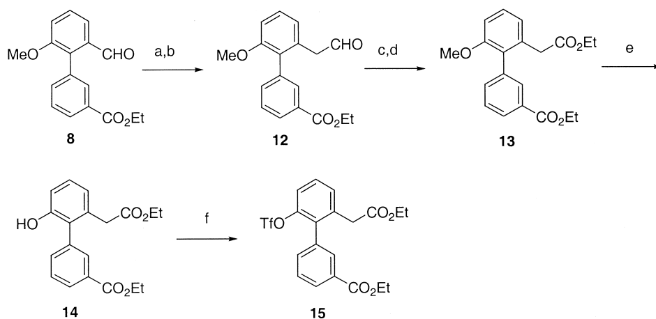
Scheme 2. Reaction conditions: (a) \text{Ph}_3\text{PCH}_2\text{OCH}_3 + \text{Cl}^- , t -BuOK, toluene, THF; (b) 1 N HCl, THF, reflux; (c) \text{NaClO}_2 , \text{H}_2\text{NSO}_3\text{H} , THF, \text{H}_2\text{O} ; (d) HCl, EtOH, reflux; (e) (\text{CH}_3)_2\text{BBr} , \text{ClCH}_2\text{CH}_2\text{Cl} ; (f) \text{TiF}_2\text{O} , DMAP, \text{CH}_2\text{Cl}_2 .
