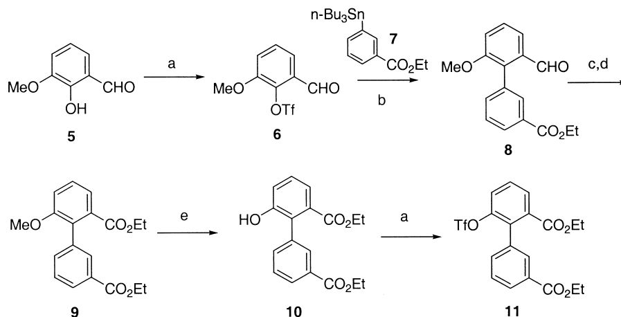
Scheme 1. Reaction conditions: (a) \text{TiF}_2\text{O} , DMAP, \text{CH}_2\text{Cl}_2 ; (b) \text{PdCl}_2(\text{PPh}_3)_2 , LiCl, DMF, 150^\circ\text{C} ; (c) \text{NaClO}_2 , \text{H}_2\text{NSO}_3\text{H} , THF, \text{H}_2\text{O} ; (d) HCl, EtOH, reflux; (e) \text{Me}_2\text{BBr} , \text{ClCH}_2\text{CH}_2\text{Cl} .
