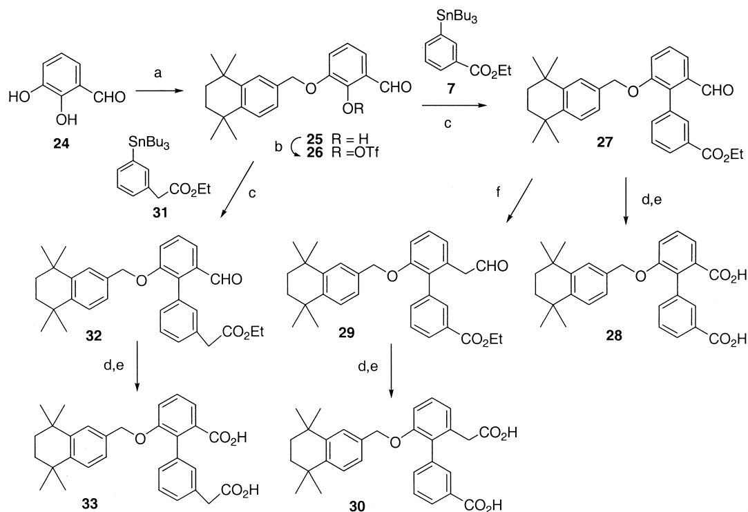
Scheme 5. Reaction conditions: (a) NaH (2.5 equiv), DMSO, 2-chloromethyl-5,5,8,8-tetramethyl-5,6,7,8-tetrahydronaphthalene; (b) Tf 2 O, DMAP, CH 2 Cl 2 ; (c) PdCl 2 (PPh 3 ) 2 , LiCl, DMF, 125 °C; (d) NaClO 2 , H 2 NSO 3 H, THF, H 2 O; (e) 2 N NaOH, CH 3 OH, THF, reflux, then 1 N HCl; (f) Ph 3 PCH 2 OCH 3 + Cl − , t -BuOK, toluene, THF; (g) 1 N HCl, THF, reflux.
