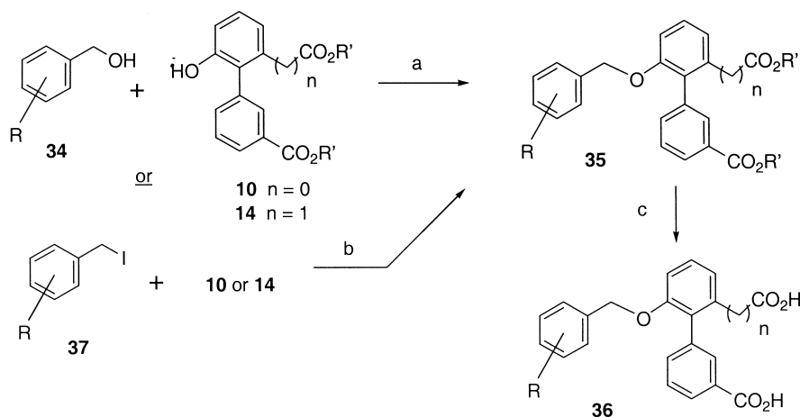
Scheme 6. Reaction conditions: (a) DIAD, PPh 3 , THF, 0 °C; (b) K 2 CO 3 , MIBK, reflux; (c) 2 N NaOH, CH 3 OH, THF, reflux, then 1 N HCl.
