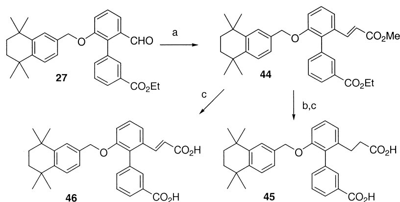
Scheme 8. Reaction conditions: (a) \text{Ph}_3\text{P}=\text{CHCO}_2\text{CH}_3 (4.4 equiv), \text{CH}_2\text{Cl}_2 ; (b) 10% \text{Pd/C} , \text{H}_2 (1 atm), \text{EtOAc} ; (c) 2 N \text{NaOH} , \text{CH}_3\text{OH} , THF, reflux, then 1 N \text{HCl} .
